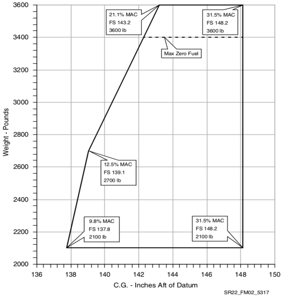
Figure 2-1: Center of Gravity Envelope
