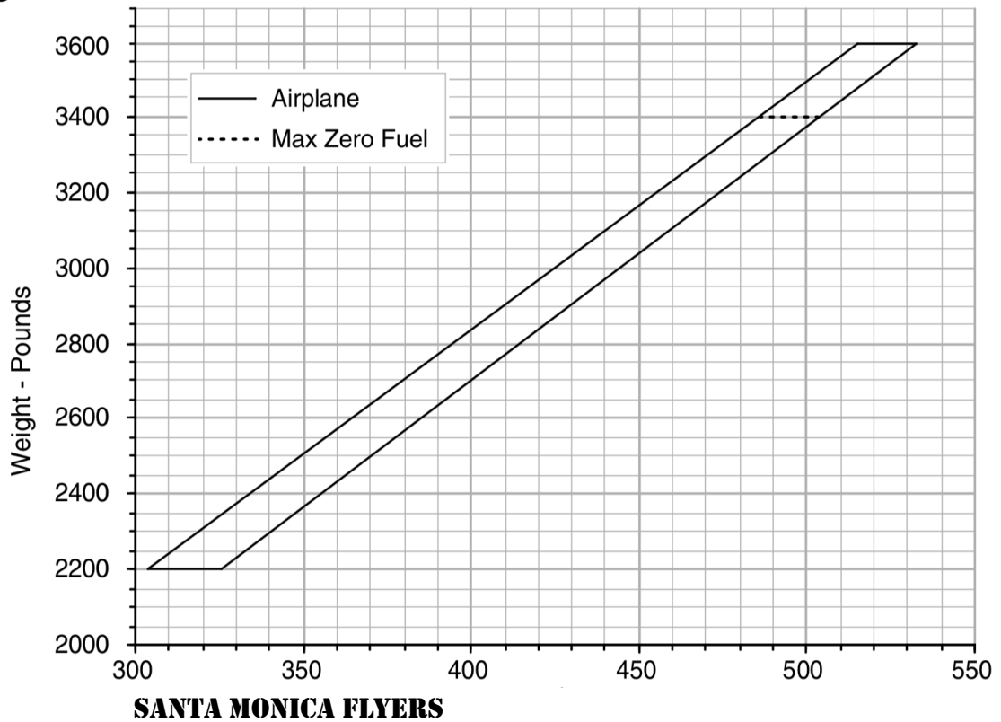
Figure 6-4: Moment Limits Chart
